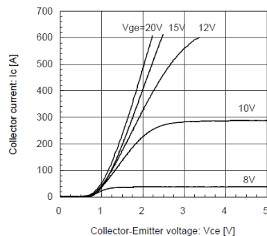
Collector current vs. Collector-Emitter voltage (typ.) T_j = 25^\circ C / \text{chip}
