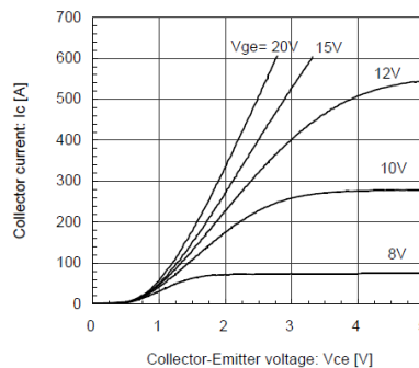
Collector current vs. Collector-Emitter voltage (typ.) T_j = 150^\circ C / \text{chip}
